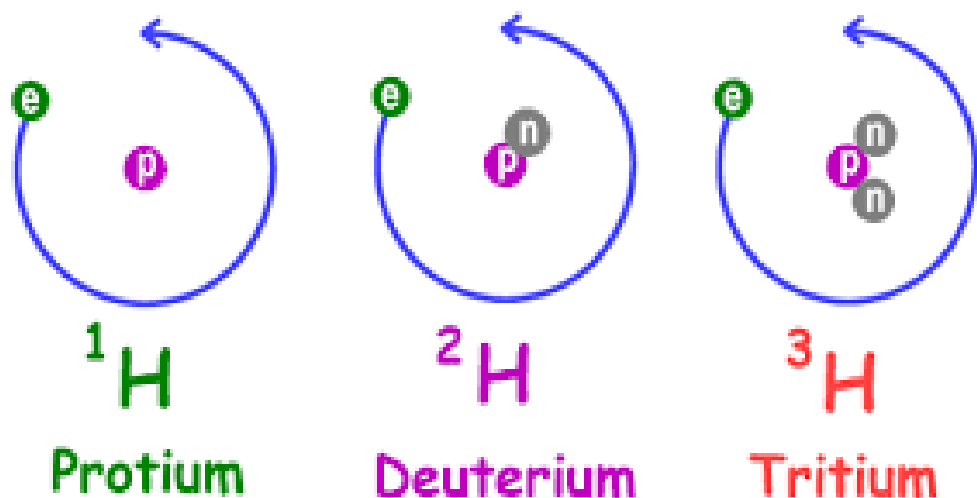
Fig 1: Three Isotopes of hydrogen
